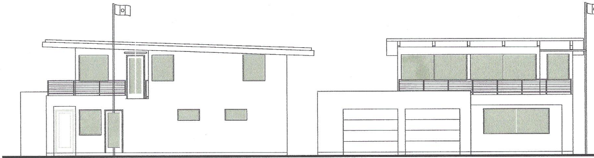
SOUTH ELEVATION
